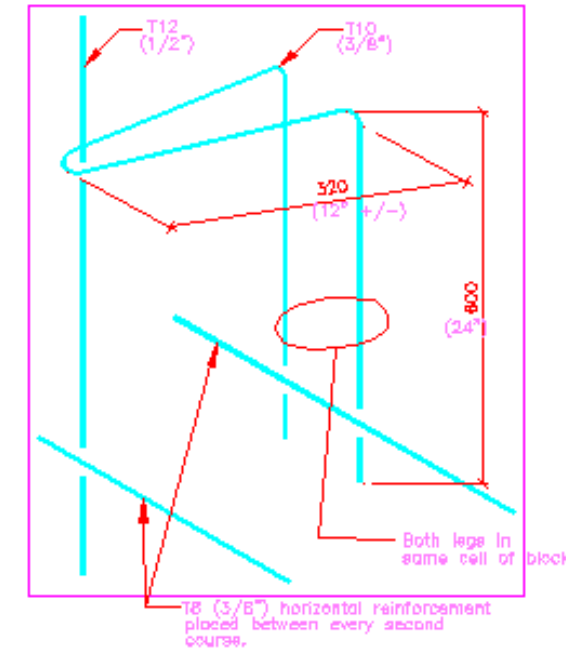
1 TYPICAL REINFORCEMENT SK1 NTS
