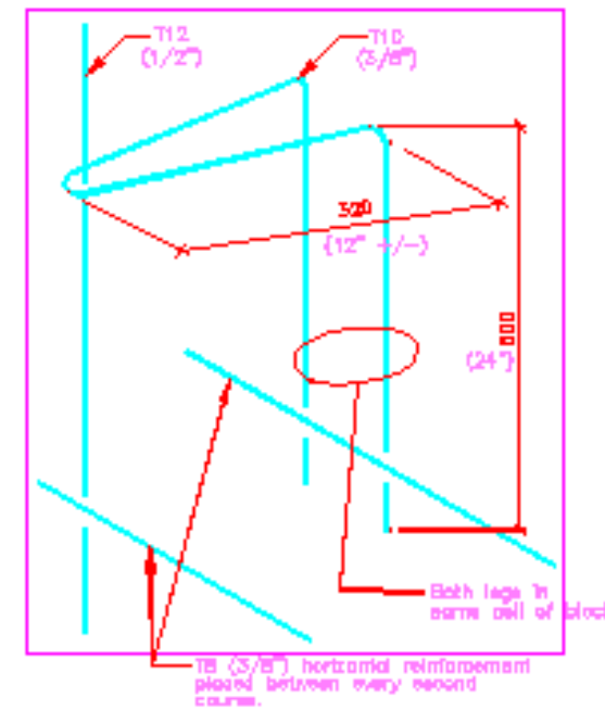
1 TYPICAL REINFORCEMENT NTS
