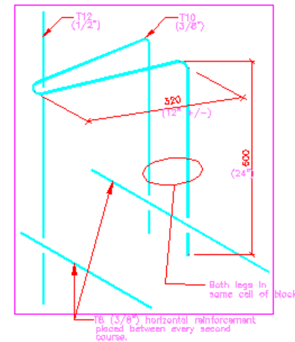
1 TYPICAL REINFORCEMENT SK1 NTS
